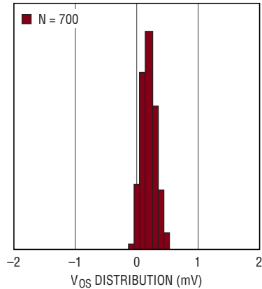
V_{\text{OS}} Distribution
