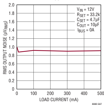
RMS Noise vs I_{\text{OUT}}
