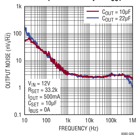
Noise Spectral Density vs C_{\text{OUT}}
