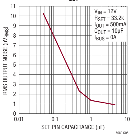
RMS Noise vs C_{\text{SET}}
