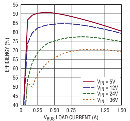
V_{BUS} Efficiency vs Load, V_{BUS} = 2.8\text{V} Pulse-Skipping Mode, f_{SW} = 900\text{kHz}
