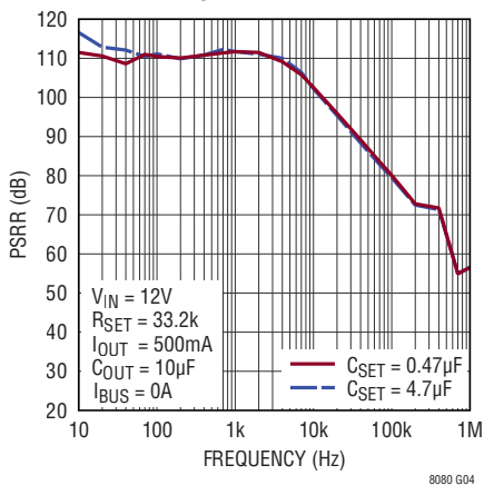
PSRR vs C_{\text{SET}}
