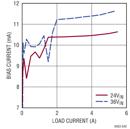
LTM8053 BIAS Current vs Load Current, V_{OUT} = 12V , BIAS = 5V
