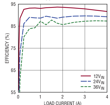
LTM8053 Efficiency vs Load Current, V_{OUT} = 8\text{V} , BIAS = 5V
