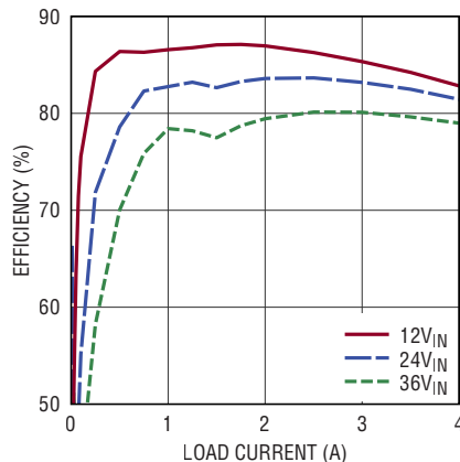
LTM8053 Efficiency vs Load Current, V_{OUT} = 2\text{V} , BIAS = 5V
