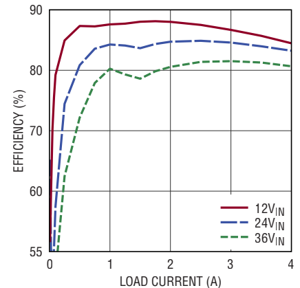
LTM8053 Efficiency vs Load Current, V_{OUT} = 2.5\text{V} , BIAS = 5V
