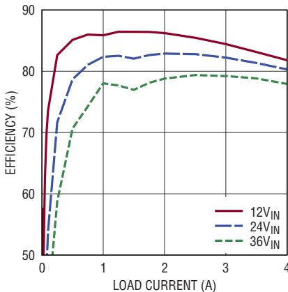
LTM8053 Efficiency vs Load Current, V_{OUT} = 1.8\text{V} , BIAS = 5V
