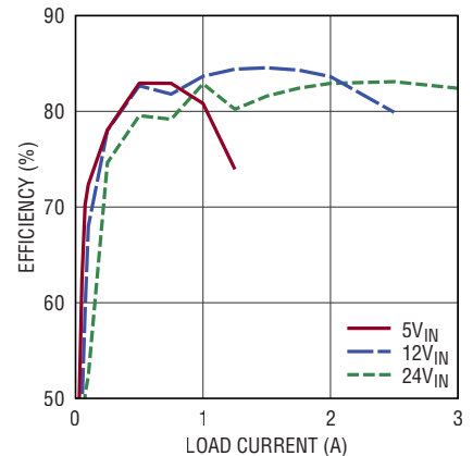
LTM8053 Efficiency vs Load Current, V_{OUT} = -12\text{V} , BIAS Tied to LTM8053 GND
