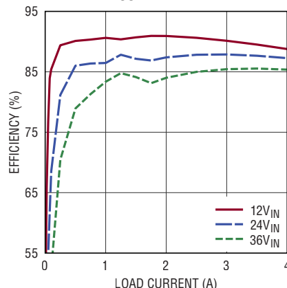
LTM8053 Efficiency vs Load Current, V_{OUT} = 5\text{V} , BIAS = 5V
