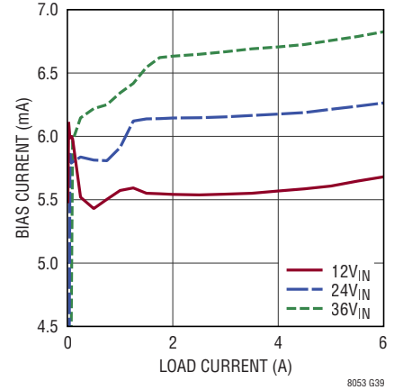
LTM8053 BIAS Current vs Load Current, V_{OUT} = 3.3V , BIAS = 5V
