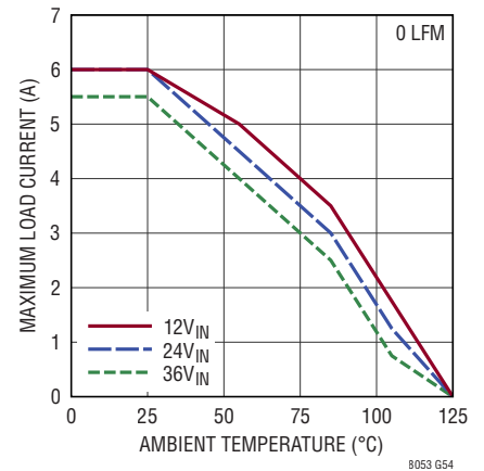
LTM8053 Derating, V_{OUT} = 3.3\text{V} , BIAS = 5V, DC1934A Demo Board
