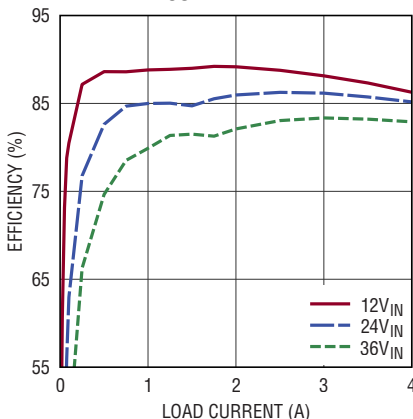
LTM8053 Efficiency vs Load Current, V_{OUT} = 3.3\text{V} , BIAS = 5V
