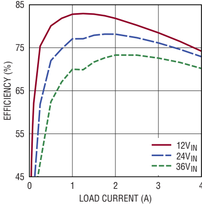
LTM8053 Efficiency vs Load Current, V_{OUT} = 0.97\text{V} , BIAS = 5V
