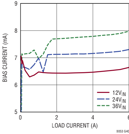
LTM8053 BIAS Current vs Load Current, V_{OUT} = 5V , BIAS = 5V
