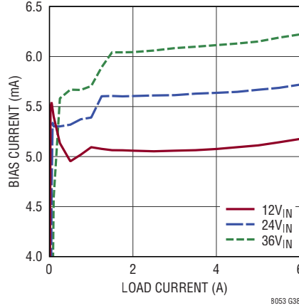
LTM8053 BIAS Current vs Load Current, V_{OUT} = 2.5V , BIAS = 5V
