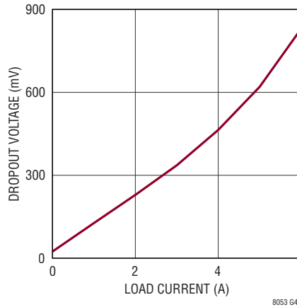
LTM8053 Dropout Voltage vs Load Current, V_{OUT} = 5V , BIAS = 5V
