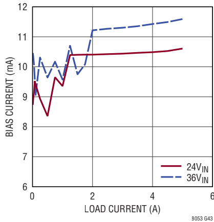
LTM8053 BIAS Current vs Load Current, V_{OUT} = 15V , BIAS = 5V
