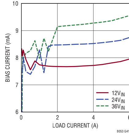
LTM8053 BIAS Current vs Load Current, V_{OUT} = 8V , BIAS = 5V
