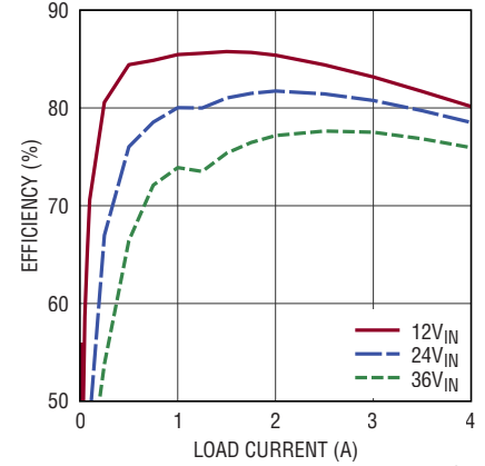
LTM8053 Efficiency vs Load Current, V_{OUT} = 1.5\text{V} , BIAS = 5V
