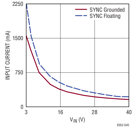
LTM8053 Input Current vs V_{IN} , V_{OUT} Short-Circuited
