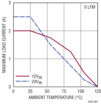
LTM8053 Derating, V_{OUT} = -12\text{V} , BIAS Tied to LTM8053 GND, DC1934A Demo Board
