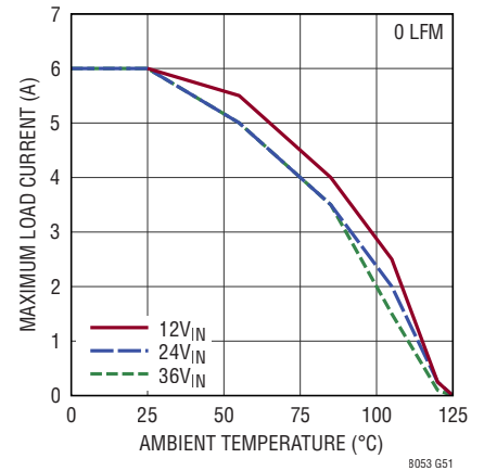
LTM8053 Derating, V_{OUT} = 1.8\text{V} , BIAS = 5V, DC1934A Demo Board
