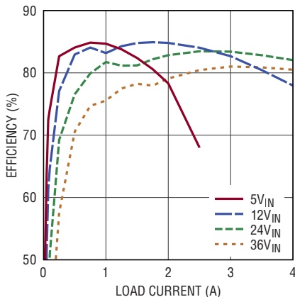
LTM8053 Efficiency vs Load Current, V_{OUT} = -5\text{V} , BIAS Tied to LTM8053 GND
