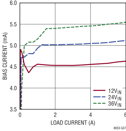
LTM8053 BIAS Current vs Load Current, V_{OUT} = 2V , BIAS = 5V
