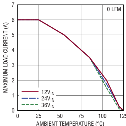
LTM8053 Derating, V_{OUT} = 2\text{V} , BIAS = 5V, DC1934A Demo Board
