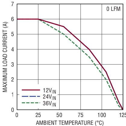
LTM8053 Derating, V_{OUT} = 1.2\text{V} , BIAS = 5V, DC1934A Demo Board
