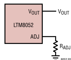
Figure 3. Voltage Regulation and Overvoltage Protection Feedback Connections
