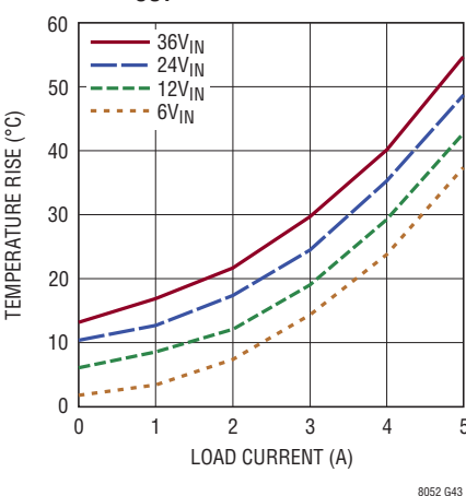
Temperature Rise vs Load Current 3.3V_{OUT}
