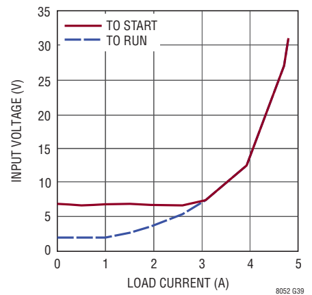
Minimum Required Input Voltage vs Load -5V_{OUT}
