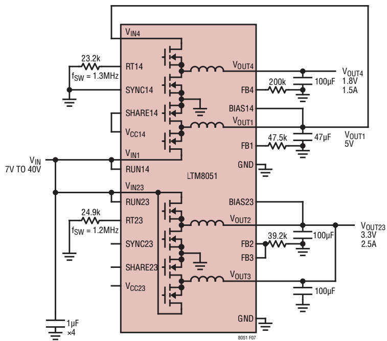
PINS NOT USED: TRSS1, TRSS2, TRSS3, TRSS4, PG1, PG2, PG3, PG4, CLKOUT14, CLKOUT23
