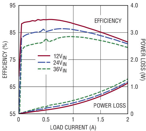
Efficiency, V_{OUT} = 2.5\text{V} BIAS = 5V, Burst Mode
