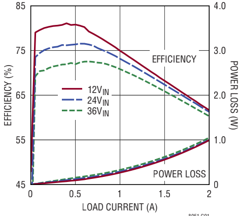
Efficiency, V_{OUT} = 0.8\text{V} BIAS = 5V
