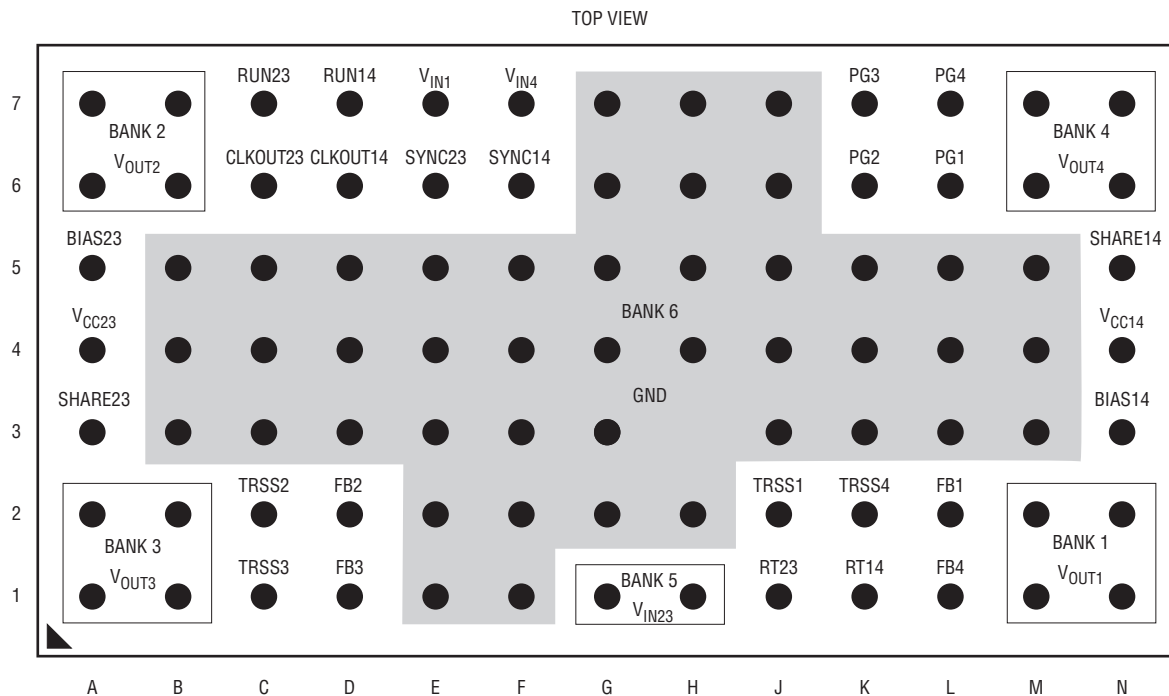
BGA PACKAGE 91-PIN (11.25mm × 6.25mm × 2.22mm)
