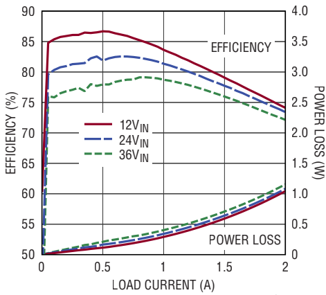
Efficiency, V_{OUT} = 1.5\text{V} BIAS = 5V, Burst Mode
