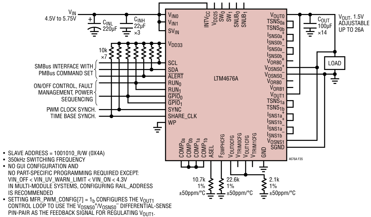
Figure 35. 26A, 1.5V Output DC/DC \mu Module Regulator with I 2 C/SMBus/PMBus Serial Interface
