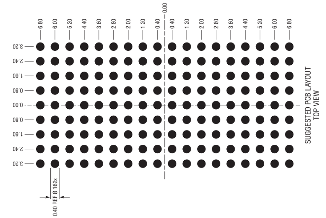
PACKAGE TOP VIEW
