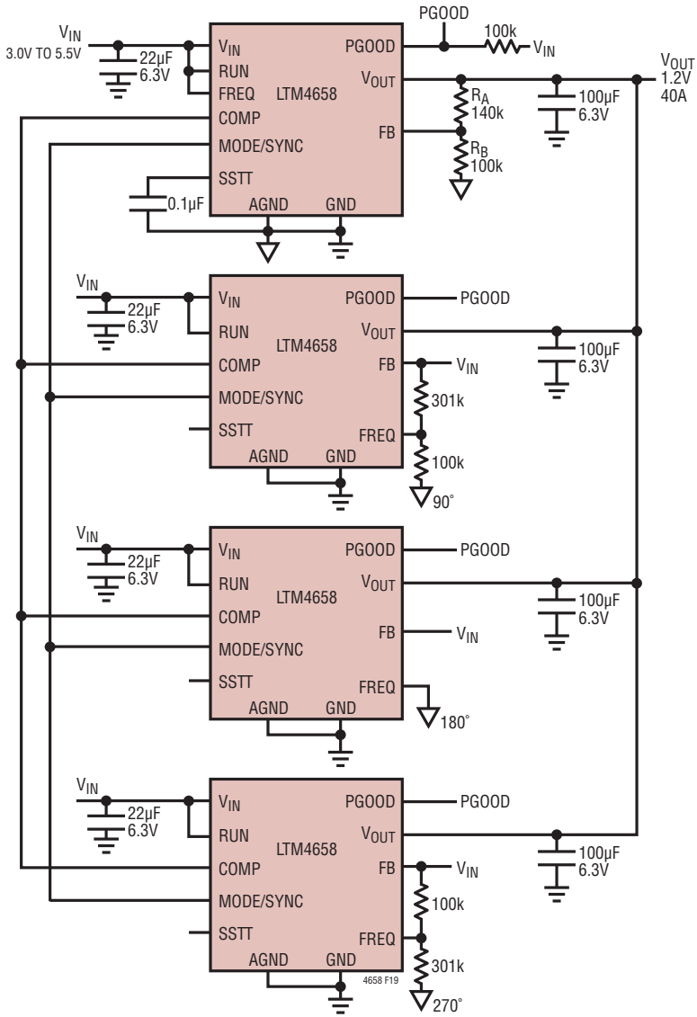
Figure 19. Four-Phase Application
