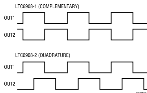
Figure 3. Output Waveforms for LTC6908-1, LTC6908-2
