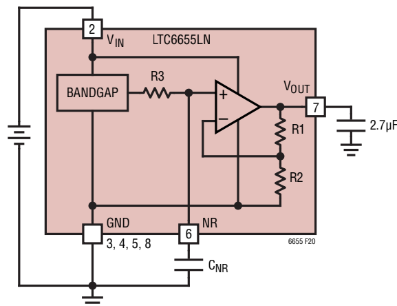
Figure 20. The LTC6655LN Typical Application Circuit
