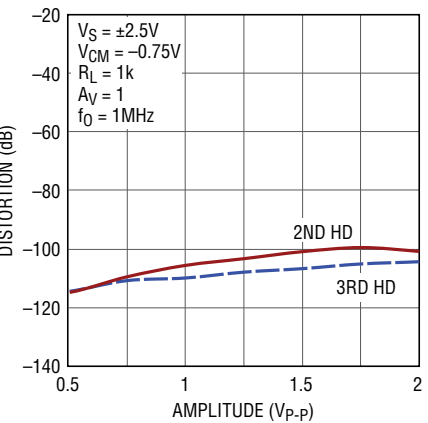
Harmonic Distortion vs Amplitude
