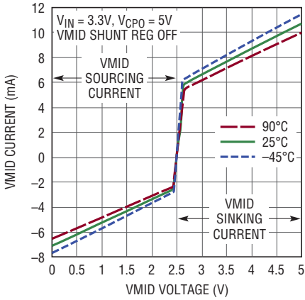
Leakage Balancer Source and Sink Capability
