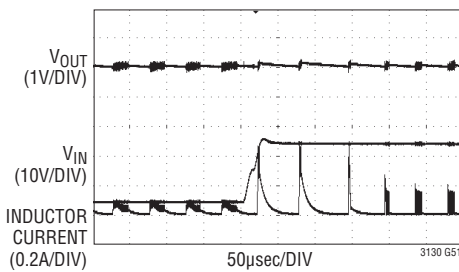
V IN Line Step Response in Burst Mode Operation
