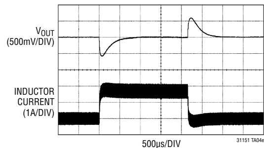
0A to 1.5A Load Step, V IN = 40V
