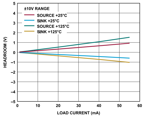
Figure 45. V_{x^+}/V^- Bipolar Headroom vs. Output Load Current
