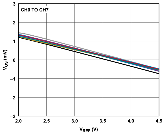
Figure 12. V_{OS} vs. V_{REF}
