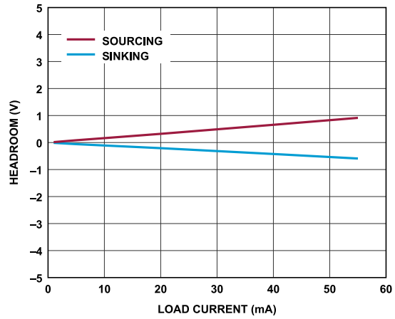
Figure 44. V_{x^+}/V^- Unipolar Headroom vs. Output Load Current
