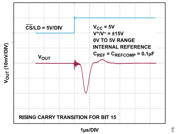
Figure 16. Glitch Impulse
