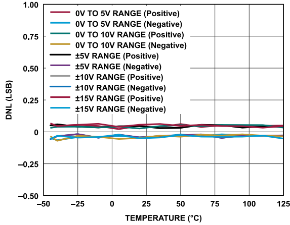
Figure 29. LTC2686-16 DNL vs. Temperature
