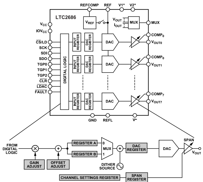
Figure 47. Block Diagram
