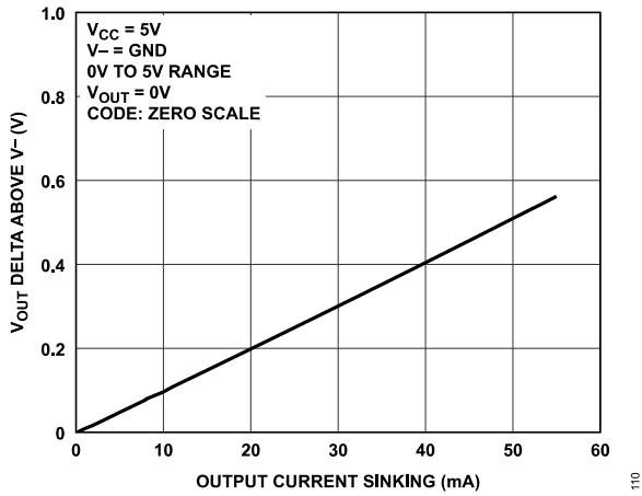
Figure 11. V_{OUT} Delta Above V^- vs. Output Current Sinking
