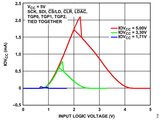
Figure 15. IOV_{CC} vs. Input Logic Voltage
