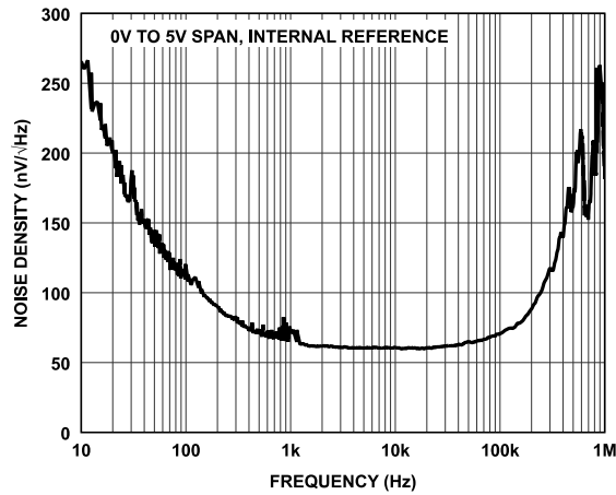
Figure 18. Noise Density vs. Frequency
