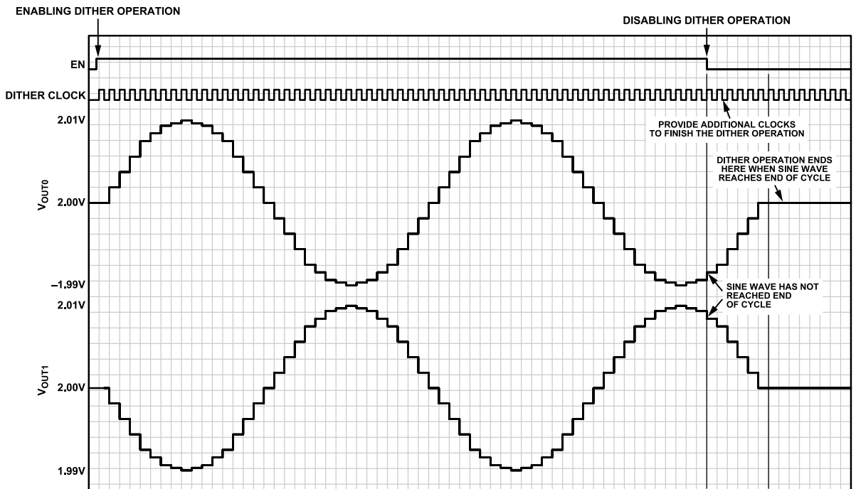
Figure 58. Termination of Sinusoidal Dither Waveforms
