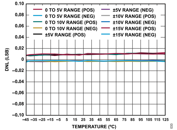
Figure 33. LTC2686-12 DNL vs. Temperature
