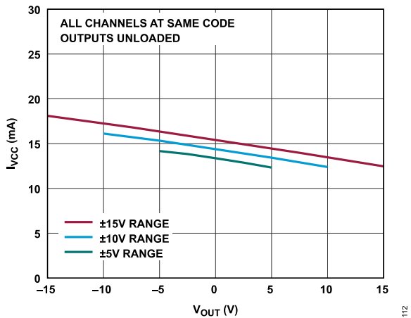
Figure 13. I_{VCC} vs. V_{OUT}
