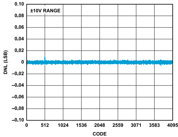
Figure 31. LTC2686-12 DNL vs. Code
