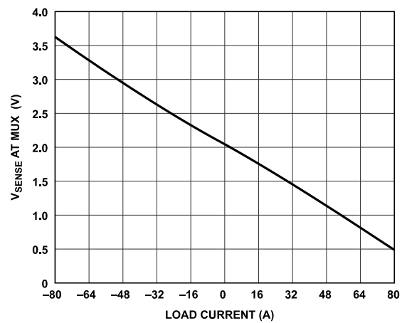
Figure 21. V_{SENSE} at MUX vs. Load Current
