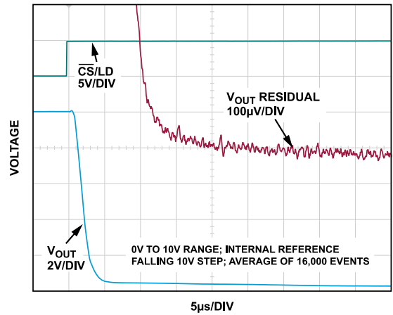
Figure 39. Settling Time, 10 V (Falling)
