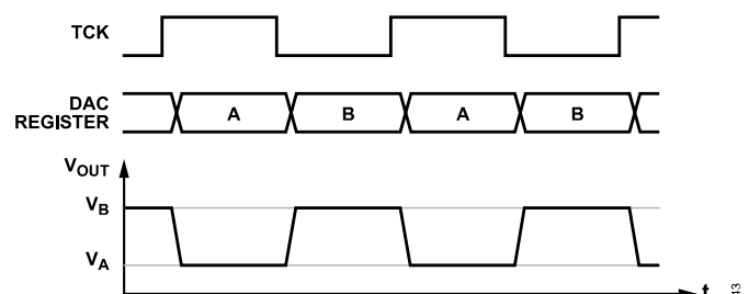
Figure 54. TCK Timing
