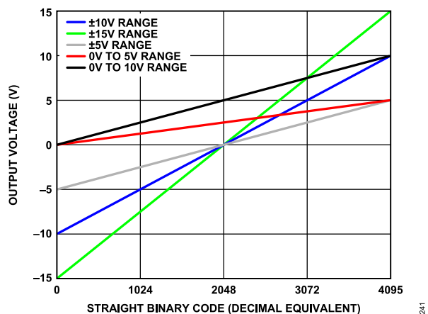
Figure 52. DAC Transfer Functions for LTC2686-12, All Voltage Spans and Bit Resolutions, Internal Reference Mode
