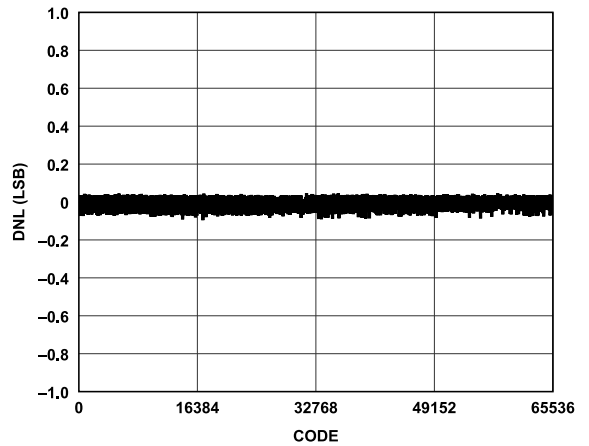
Figure 27. LTC2686-16 DNL vs. Code
