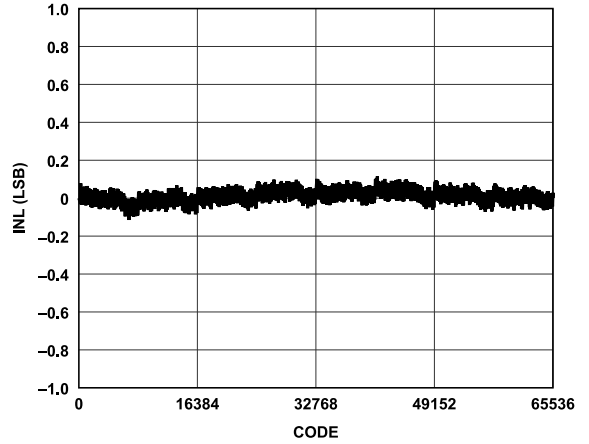
Figure 26. LTC2686-16 INL vs. Code
