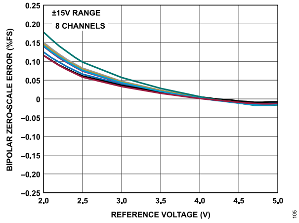
Figure 6. Bipolar Zero-Scale Error vs. V_{REF}
