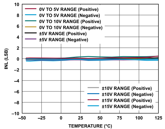
Figure 28. LTC2686-16 INL vs. Temperature
