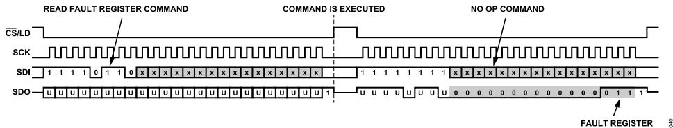
Figure 50. Typical Read Command Sequence for 24-Bit Words
