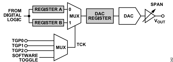
Figure 53. Toggle Operation
