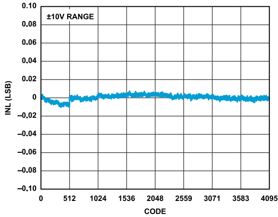
Figure 30. LTC2686-12 INL vs. Code
