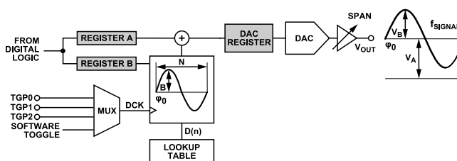
Figure 55. Dither Signal Operation
