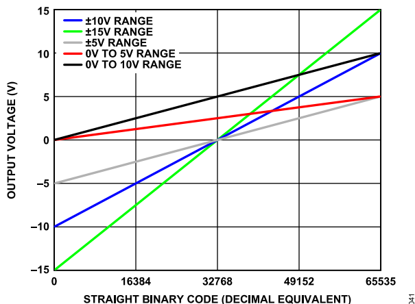
Figure 51. DAC Transfer Functions for LTC2686-16, All Voltage Spans and Bit Resolutions, Internal Reference Mode
