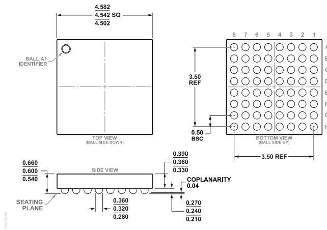
Figure 62. 64-Ball Wafer Level Chip Package [WLCSP] (CB-64-5) Dimensions shown in millimeters
