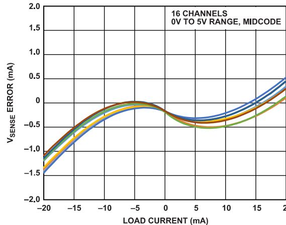
Figure 46. V_{SENSE} Error vs. Load Current from Equation 5
