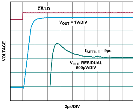
0V TO 5V RANGE; INTERNAL REFERENCE RISING 5V STEP; AVERAGE OF 64 EVENTS. FALLING SETTLE IS SIMILAR OR BETTER. SUBTRACT 100ns FIXTURE DELAY FROM SETTLE WAVEFORM.
