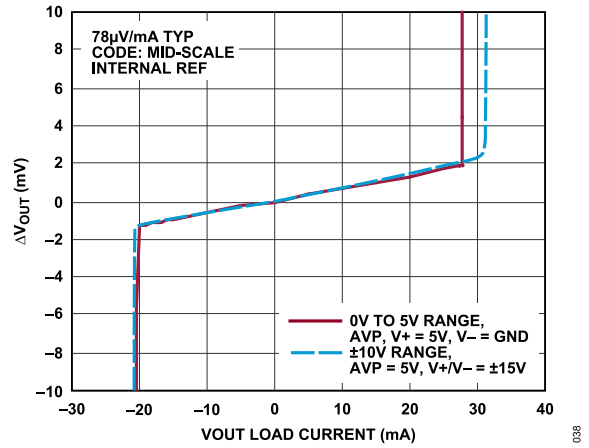
Figure 25. Load Regulation
