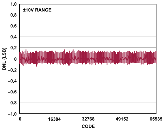
Figure 27. Differential Nonlinearity (DNL)
