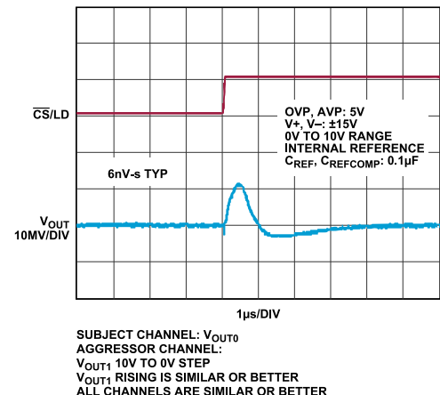
Figure 20. DAC-to-DAC Crosstalk
