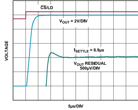
0V TO 10V RANGE; INTERNAL REFERENCE RISING 10V STEP; AVERAGE OF 64 EVENTS. FALLING SETTLE IS SIMILAR OR BETTER. SUBTRACT 100ns FIXTURE DELAY FROM SETTLE WAVEFORM.
