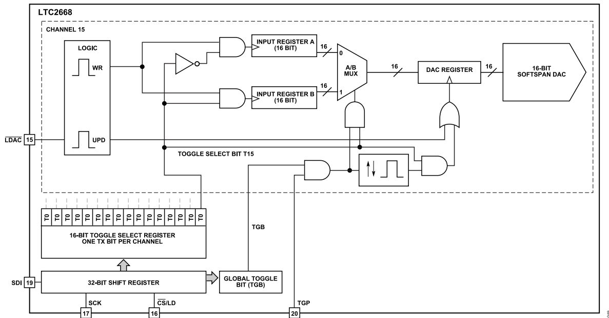
Figure 46. Simplified Toggle Block Diagram—Conceptual Only, Actual Circuit May Differ
