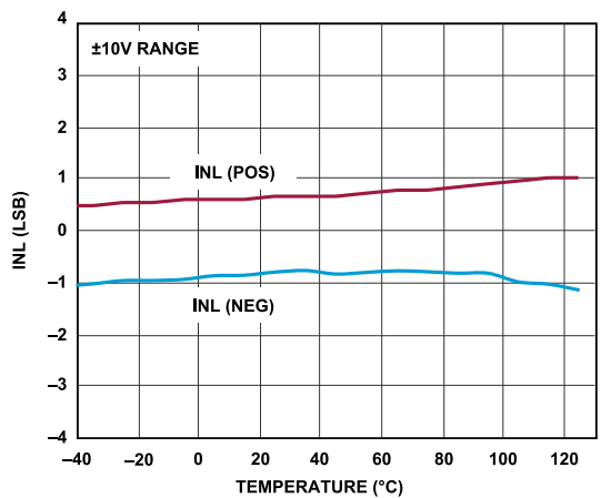
Figure 28. INL vs. Temperature
