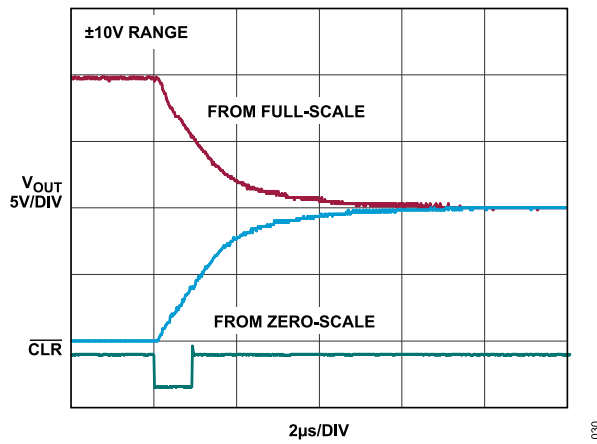
Figure 17. Hardware \overline{CLR} to Midscale
