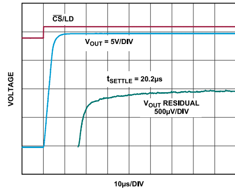
±10V RANGE; INTERNAL REFERENCE RISING 20V STEP; AVERAGE OF 64 EVENTS. FALLING SETTLE IS SIMILAR OR BETTER. SUBTRACT 100ns FIXTURE DELAY FROM SETTLE WAVEFORM.
