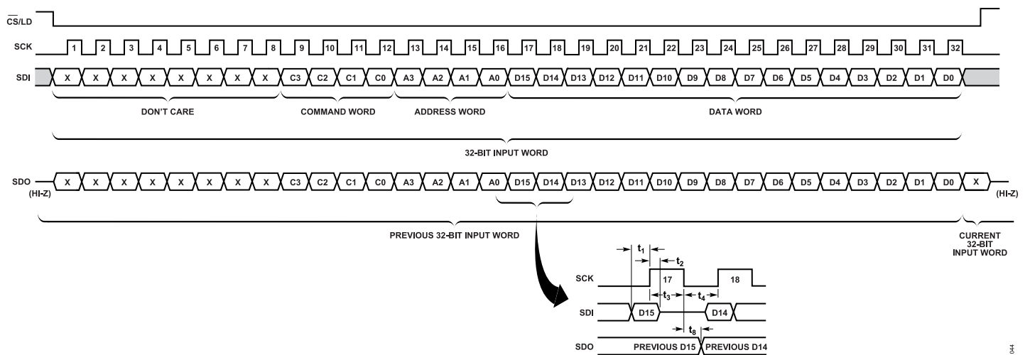
Figure 41. LTC2668-16 32-Bit Load Sequence, LTC2668-12 SDI/SDO Data-Word Is 12-Bit Input Code + 4 Don't Care Bits
