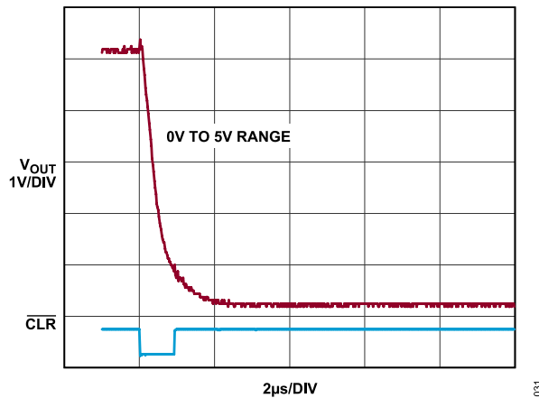
Figure 18. Hardware \overline{CLR} to Zero Scale
