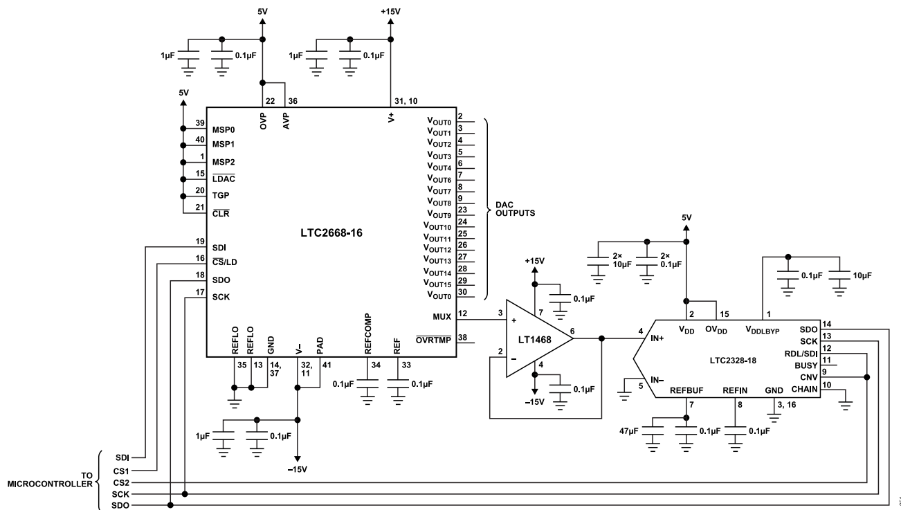
Figure 51. Using the Analog Multiplexer to Measure DAC Output Voltages Up to \pm 10.24 V; Independent ADC Reference Cross-Checks LTC2668 Internal Reference
