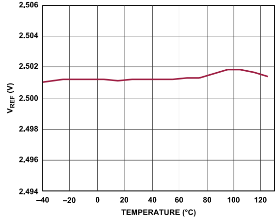
Figure 7. Reference Output vs. Temperature
