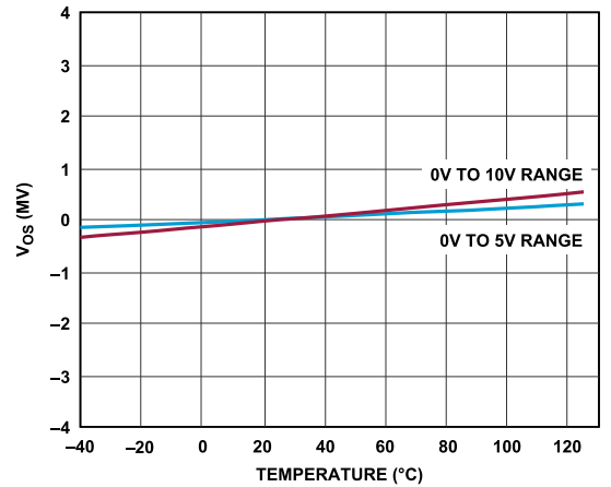
Figure 8. Unipolar Offset vs. Temperature
