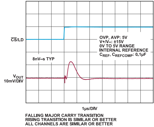
Figure 19. Midscale Glitch Impulse
