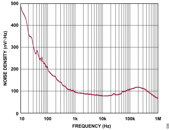
Figure 22. Noise Density vs. Frequency
