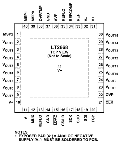
Figure 3. Pin Configuration
