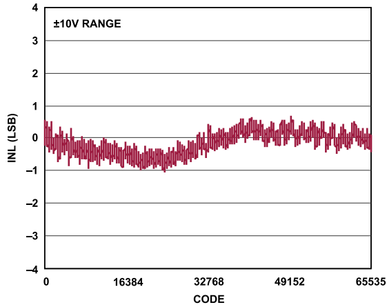
Figure 26. Integral Nonlinearity (INL)
