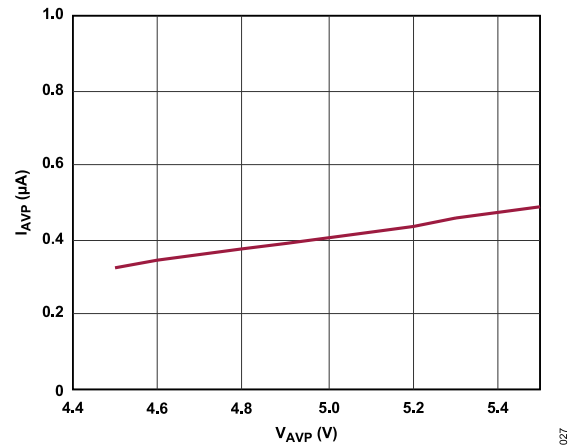
Figure 14. AVP Shutdown Current vs. AVP
