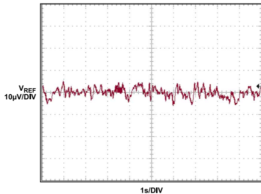
Figure 23. Output 0.1 Hz to 10 Hz Voltage Noise
