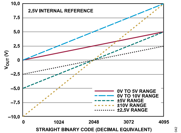
Figure 39. LTC2668-12 Transfer Function
