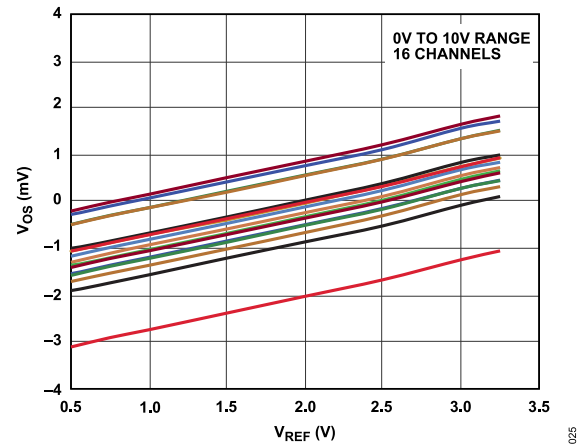
Figure 12. Unipolar Offset vs. Reference Input
