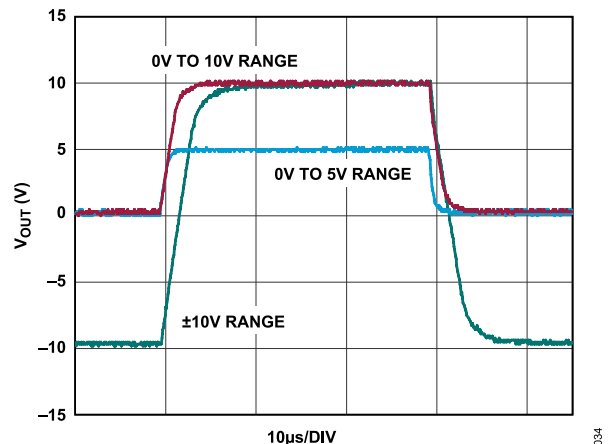
Figure 21. Large Signal Response
