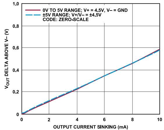
Figure 9. Headroom to V - Rail vs. Output Current
