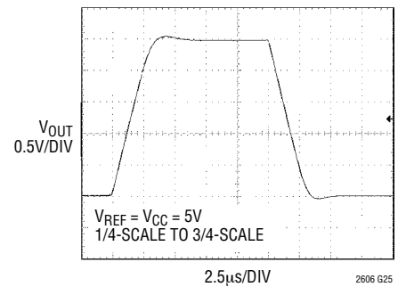
Large-Signal Response
