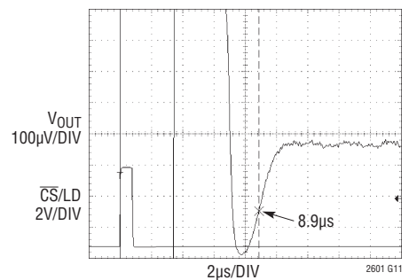
Settling to \pm 1\text{LSB}
