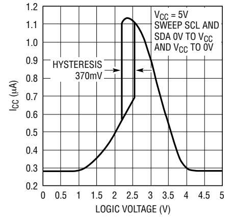
Supply Current vs Logic Voltage
