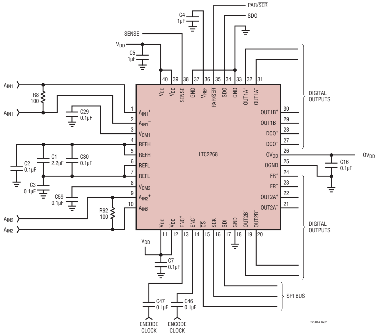
LTC2268 Schematic
