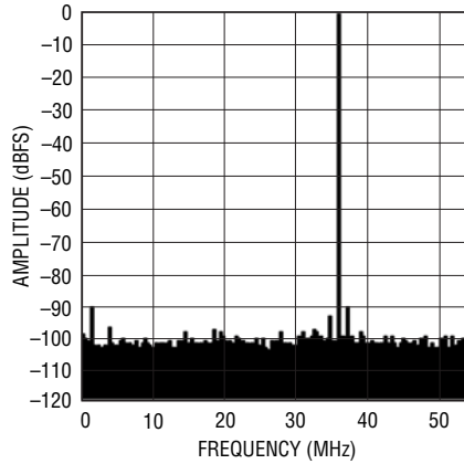
LTC2267-14: 8k Point FFT, f IN = 70MHz, -1dBFS, 105Mpsps
