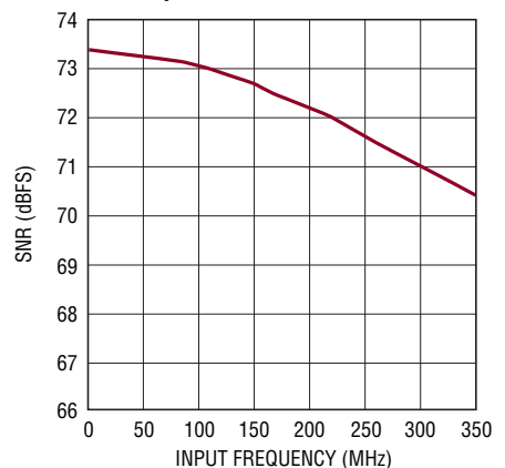
LTC2267-14: SNR vs Input Frequency, -1dB, 2V Range, 105Mpsps
