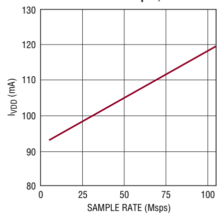
LTC2267-14: I VDD vs Sample Rate, 5MHz Sine Wave Input, -1dB
