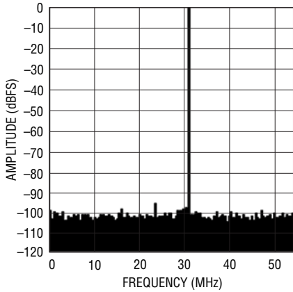
LTC2267-14: 8k Point FFT, f IN = 30MHz, -1dBFS, 105Mpsps
