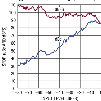
LTC2267-14: SFDR vs Input Level, f IN = 70MHz, 2V Range, 105Mpsps
