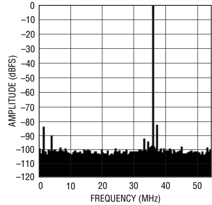
LTC2267-14: 8k Point FFT, f IN = 140MHz, -1dBFS, 105Mpsps
