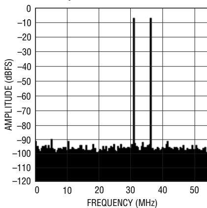
LTC2267-14: 8k Point 2-Tone FFT, f IN = 70MHz, 75MHz, -1dBFS, 105Mpsps
