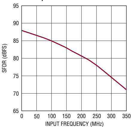
LTC2267-14: SFDR vs Input Frequency, -1dB, 2V Range, 105Mpsps
