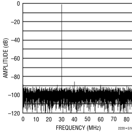
LTC2220: 8192 Point FFT, f_{IN} = 30\text{MHz} , -1\text{dB} , 1\text{V} Range, LVDS Mode
