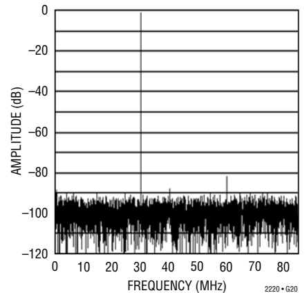
LTC2220: 8192 Point FFT, f_{IN} = 140\text{MHz} , -1\text{dB} , 1\text{V} Range, LVDS Mode
