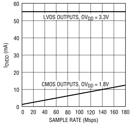
LTC2221: I_{OVD} vs Sample Rate, 5MHz Sine Wave Input, -1\text{dB}
