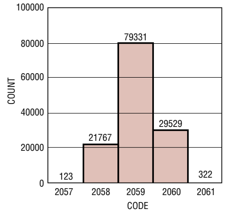
LTC2221: Shorted Input Noise Histogram
