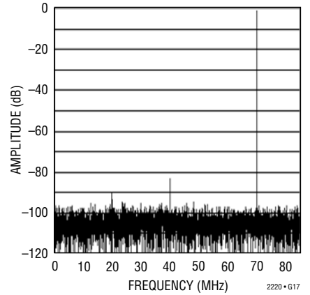
LTC2220: 8192 Point FFT, f_{IN} = 70\text{MHz} , -1\text{dB} , 2\text{V} Range, LVDS Mode
