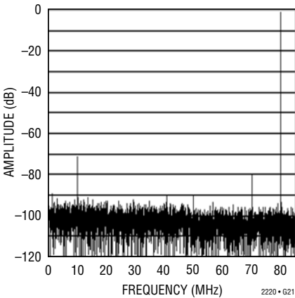
LTC2220: 8192 Point FFT, f_{IN} = 250\text{MHz} , -1\text{dB} , 2\text{V} Range, LVDS Mode
