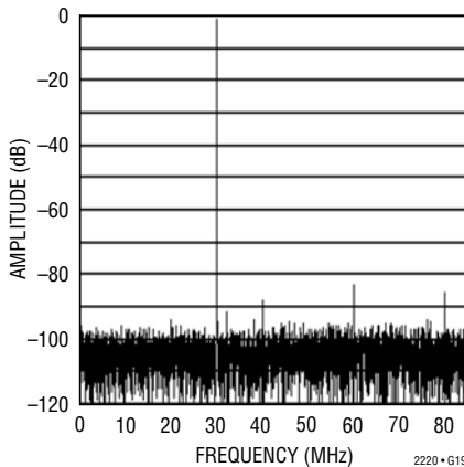
LTC2220: 8192 Point FFT, f_{IN} = 140\text{MHz} , -1\text{dB} , 2\text{V} Range, LVDS Mode
