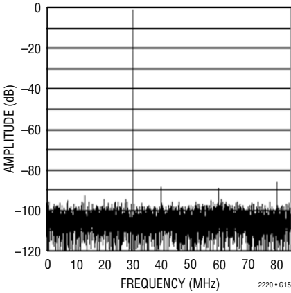
LTC2220: 8192 Point FFT, f_{IN} = 30\text{MHz} , -1\text{dB} , 2\text{V} Range, LVDS Mode
