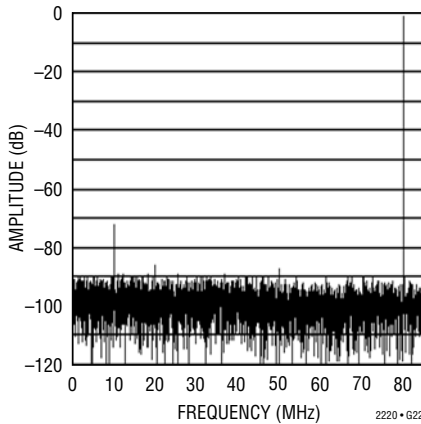
LTC2220: 8192 Point FFT, f_{IN} = 250\text{MHz} , -1\text{dB} , 1\text{V} Range, LVDS Mode
