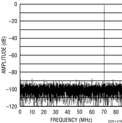
LTC2220: 8192 Point FFT, f_{IN} = 70\text{MHz} , -1\text{dB} , 1\text{V} Range, LVDS Mode
