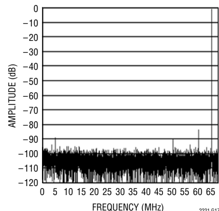
LTC2221: 8192 Point FFT, f IN = 70MHz, -1dB, 2V Range, LVDS Mode
