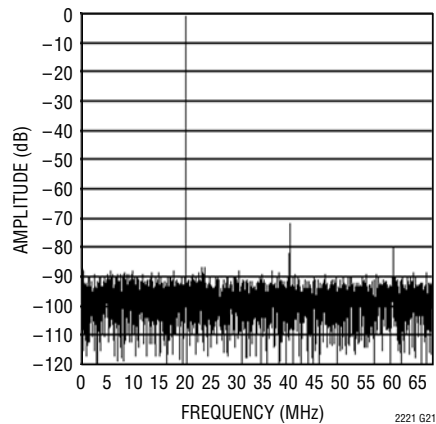
LTC2221: 8192 Point FFT, f IN = 250MHz, -1dB, 2V Range, LVDS Mode
