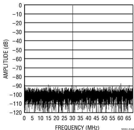
LTC2221: 8192 Point FFT, f IN = 30MHz, -1dB, 1V Range, LVDS Mode
