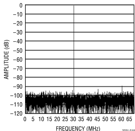
LTC2221: 8192 Point FFT, f IN = 30MHz, -1dB, 2V Range, LVDS Mode
