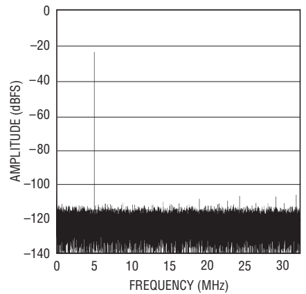
LTC2205: 64K Point FFT, f_{IN} = 5.1\text{MHz} , -25\text{dBFS} , \text{PGA} = 0 , \text{DITH} = 0
