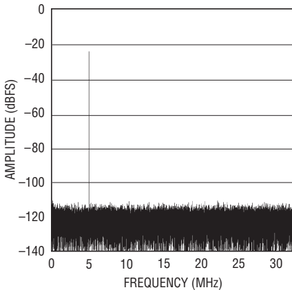
LTC2205: 64K Point FFT, f_{IN} = 5.1\text{MHz} , -25\text{dBFS} , \text{PGA} = 0 , \text{DITH} = 1
