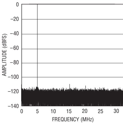
LTC2205: 64K Point FFT, f_{IN} = 5.1\text{MHz} , -1\text{dBFS} , \text{PGA} = 0 , \text{DITH} = 0
