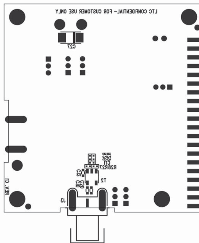
Silkscreen Bottom
