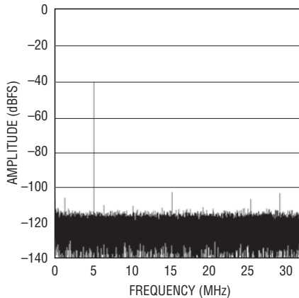
LTC2205: 64K Point FFT, f_{IN} = 5.1\text{MHz} , -40\text{dBFS} , \text{PGA} = 0 , \text{DITH} = 0
