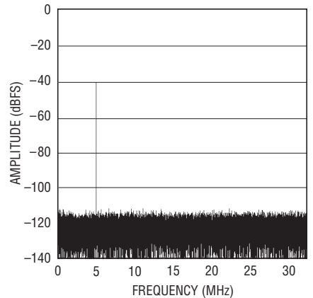
LTC2205: 64K Point FFT, f_{IN} = 5.1\text{MHz} , -40\text{dBFS} , \text{PGA} = 0 , \text{DITH} = 1
