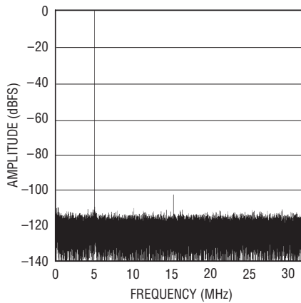
LTC2205: 64K Point FFT, 65Mps, f_{IN} = 5.1\text{MHz} , -1\text{dBFS} , \text{PGA} = 1 , \text{DITH} = 0
