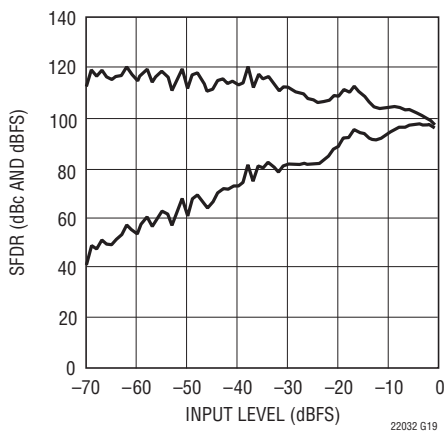
LTC2203: SFDR vs Input Level, f_{IN} = 12.7\text{MHz} , \text{PGA} = 0 , Dither "On"
