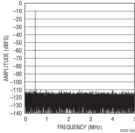
LTC2202: 32K Point FFT, f_{IN} = 30.5\text{MHz} , -10\text{dBFS} , \text{PGA} = 1
