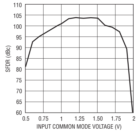
LTC2203: SFDR vs Input Common Mode Voltage, f IN = 5MHz, -1dBFS, PGA = 0
