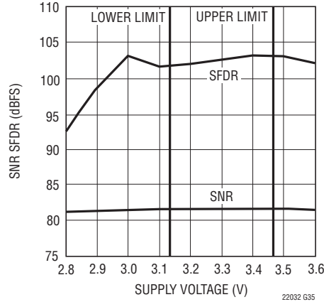
LTC2203: SNR and SFDR vs Supply Voltage (V DD ), f IN = 5MHz
