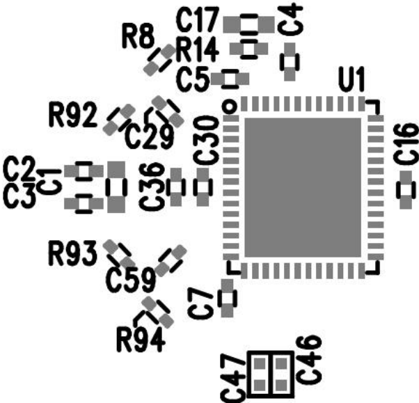
Silkscreen Top
