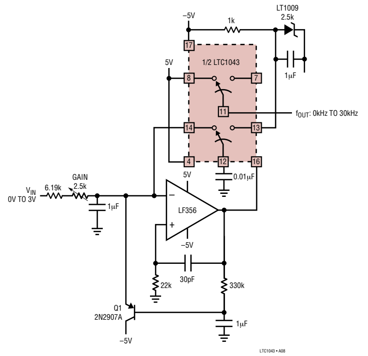
0.005% V/F Converter
