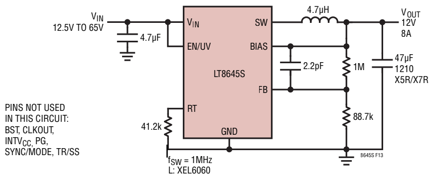
Figure 13. 12V, 8A Step-Down Converter
