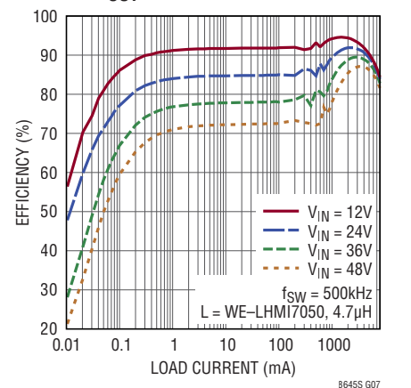
LT8645S Low Load Efficiency at 3.3V OUT
