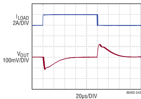
LT8640S Transient Response; Internal Compensation
