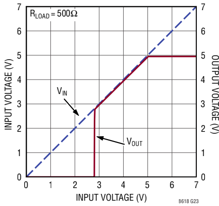
Start-Up Dropout
