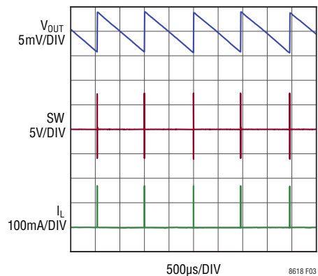
Figure 3. Burst Mode Operation (LT8618C)
