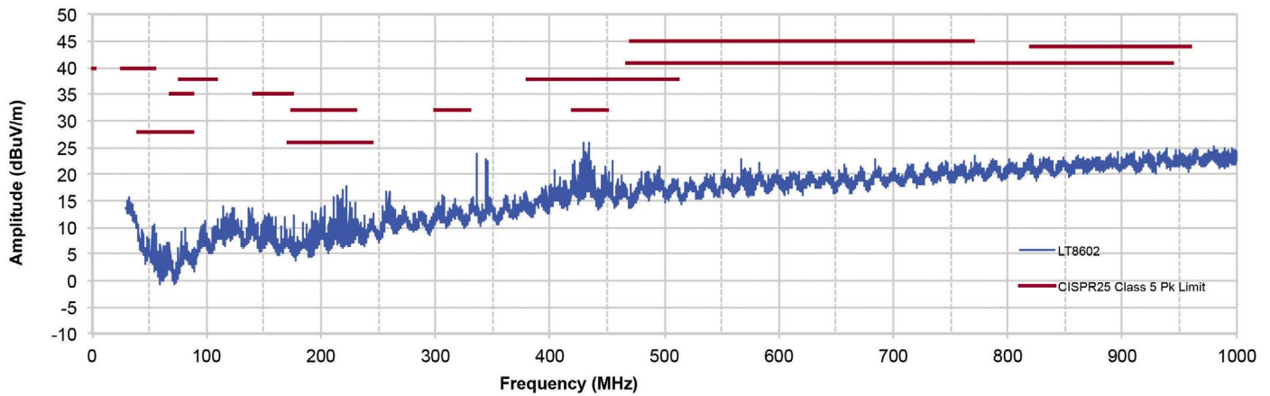
Horizontal Polarization
