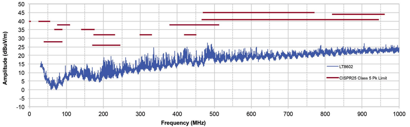
Vertical Polarization
