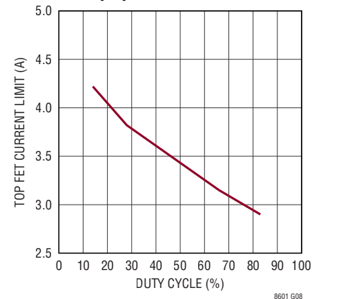
Channel 2 Peak Current Limit vs Duty Cycle
