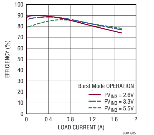
LV Channel Efficiency vs Load V_{OUT3} = 1.2\text{V} , f_{SW} = 2\text{MHz}
