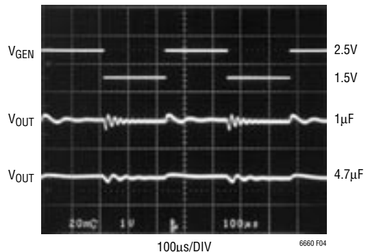
Figure 4. I_{OUT} = 1mA
