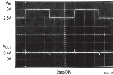
Figure 4. Output Response to \pm 0.5 V Input Step
