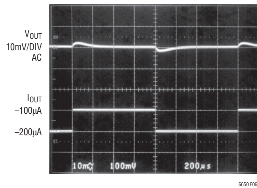
Figure 6. Output Response to Current-Sourcing Load Step ( -100\mu A to -200\mu A)
