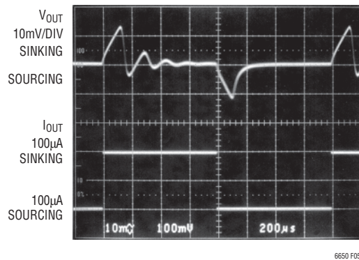
Figure 5. Output Response to Bidirectional Load Step ( 100\mu A to -100\mu A)
