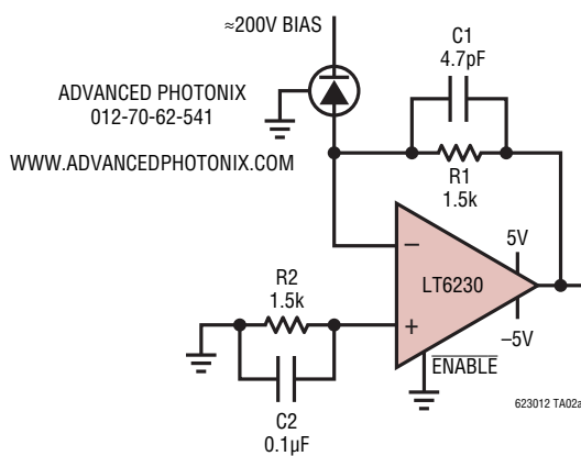
Low Power Avalanche Photodiode Transimpedance Amplifier I_S = 3.3mA
