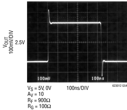
Small-Signal Response
