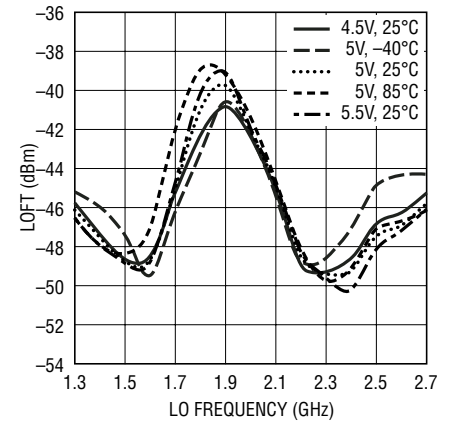
LO to RF Output Feed-Through vs LO Frequency
