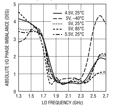
Absolute I/Q Phase Imbalance vs LO Frequency
