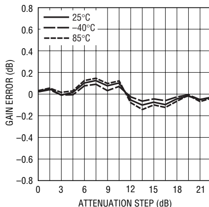
Gain Error vs Attenuation at 100MHz, R_{OUT} = 200\Omega
