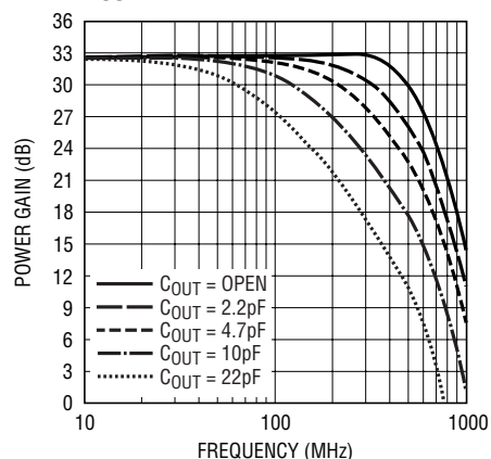
Max Gain Frequency Response with C_{OUT} as Parameter, R_{OUT} = 200\Omega
