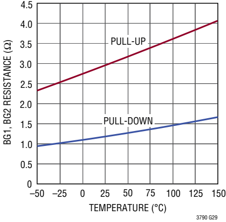
BG1, BG2 Driver On-Resistance vs Temperature
