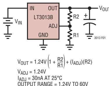
Figure 1. Adjustable Operation
