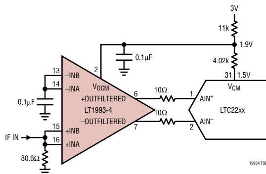
Figure 9. Level Shifting 3V ADC V_{OCM} Voltage for Improved SFDR
