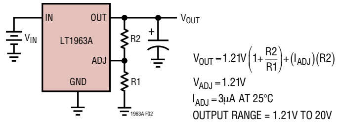
Figure 2. Adjustable Operation
