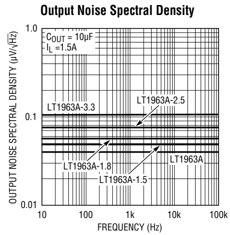
LT1963A-3.3 10Hz to 100kHz Output Noise
