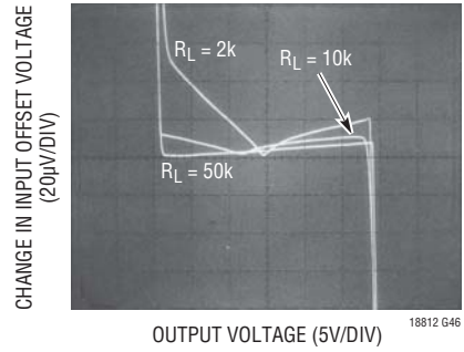
Open-Loop Gain
