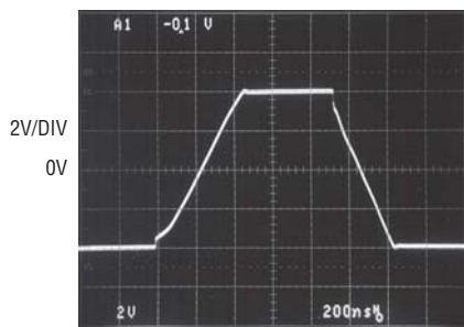
\pm 5V Large-Signal Response
