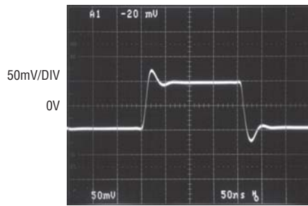
\pm 5V Small-Signal Response
