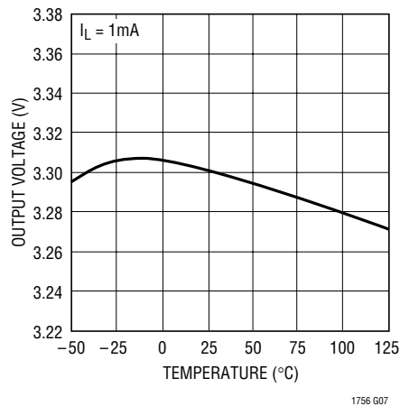
LT1764A-3.3 Output Voltage
