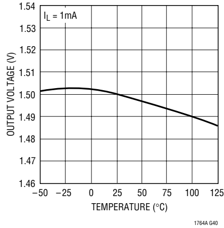
LT1764A-1.5 Output Voltage
