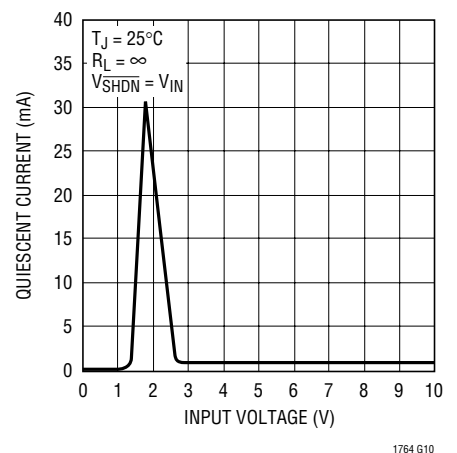
LT1764A-2.5 Quiescent Current
