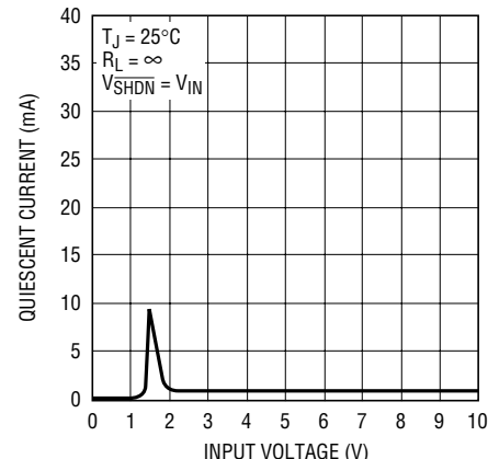
LT1764-1.8 Quiescent Current
