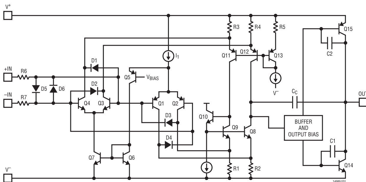
Figure 1. LT1498 Simplified Schematic Diagram
