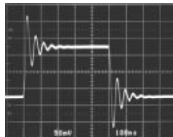
Small-Signal Transient ( A_V = -1, C_L = 200\text{pF} )
