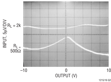
Open-Loop Gain, VS = ±15V
