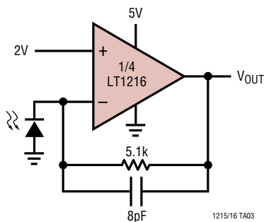
I TO V BANDWIDTH = 7MHz
